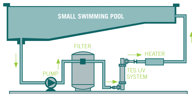
TYPICAL INSTALLATION OF TES FOR SWIMMING POOL
