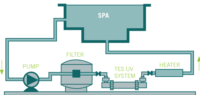
TYPICAL INSTALLATION OF TES FOR SPA
