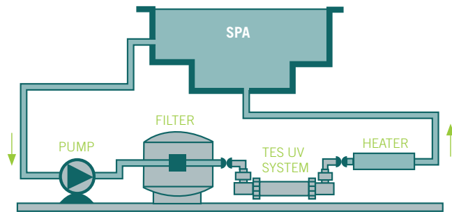
TYPICAL INSTALLATION OF TES FOR SPA
