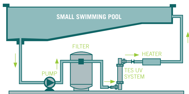
TYPICAL INSTALLATION OF TES FOR SWIMMING POOL
